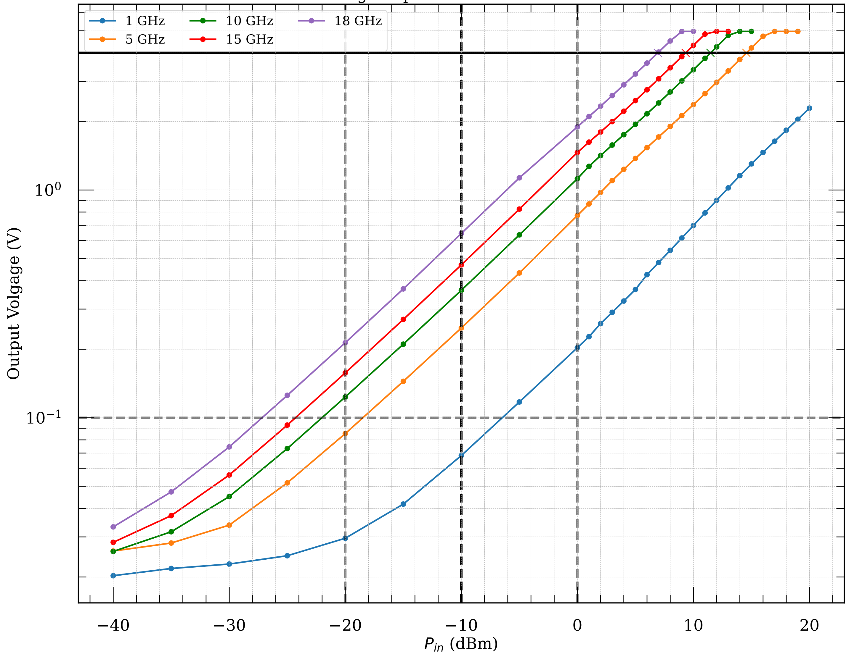
Measured voltage-to-power curve of detector module024
